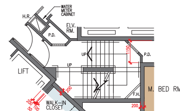
PART PLAN AT 30/F-41/F 30樓至41樓 局部平面圖
